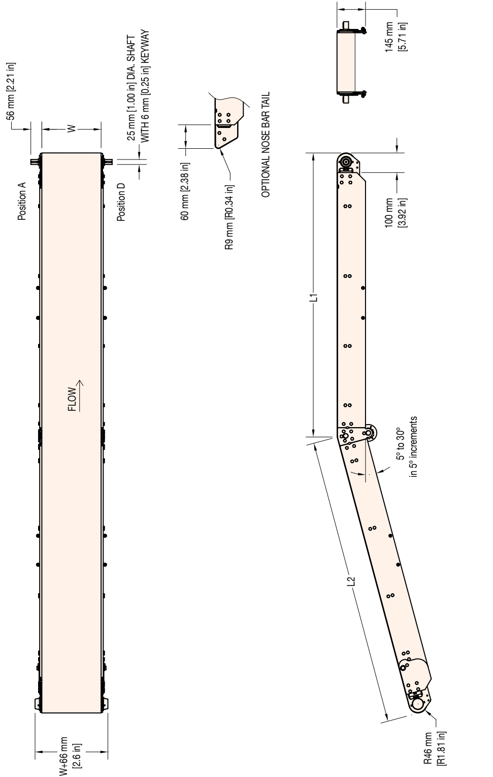
W = Conveyor Belt Width Dim = mm (in)
